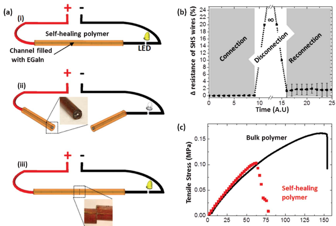
Fig. 4 Self-healing stretchable wire. (a) Schematic demonstrating the severing and restoration of the conduction path. (b) Relative resistance of the wire during a severing–restoration sequence. The researchers attribute the slight increase in resistance after restoration to imperfect alignment of the channel interfaces or displacement of small amounts of metal during the severing process. (c) Mechanical characterization of the wire before being cut (continuous line) and after being restored (discrete points). The self-healed polymer fails at a lower strain ( \sim 60\% ). Image reproduced from ref. 7.
