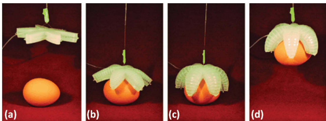
Fig. 5 Starfish-like structure of layered elastomeric materials. (a–d) Actuation of the pneumatic network embedded in the topmost layer of the structure causes the structure to curl downward, enabling gripping of an uncooked egg; grip is sufficient to support the weight of the egg upon lifting of the end-effector. Image reproduced from ref. 20.
