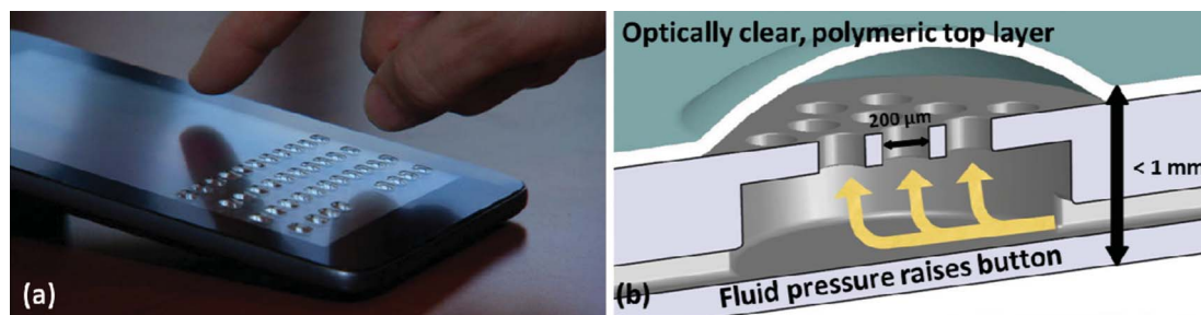
Fig. 1 (a) Three-dimensional, transparent, fluid-filled buttons overtop a touchscreen; buttons automatically rise from the screen when needed for typing and recede after typing is complete. (b) Buttons result from an embedded microfluidic network; an increase in fluid pressure causes fluid movement through the microholes, forcing the polymeric layer to bulge outward and creating a series of depressible buttons. Images reproduced from ref. 11 and 12.
