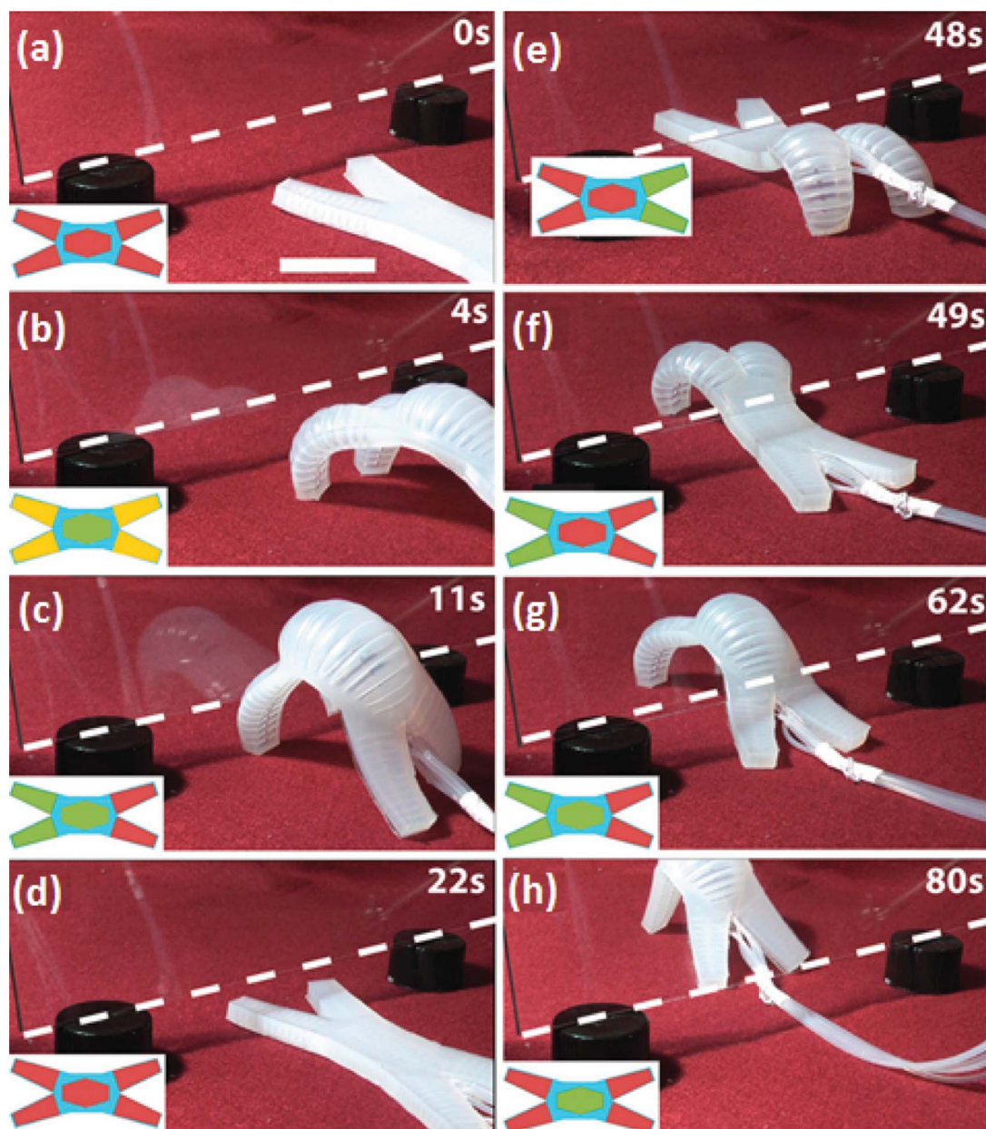
Fig. 6 Four-legged soft robot made of layered elastomeric materials, with separate pneumatic networks embedded in the spine and each of the legs. (a)–(h) Pressurization/depressurization of these embedded networks in strategic sequences moves the robot, and enables the robot to pass under a vertical plate of glass raised 2 cm off the ground (bottom edge indicated by the dashed white line). Image reproduced from ref. 21.
