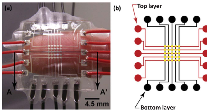
Fig. 3 Flexible microfluidic sensor that uses capacitance changes between liquid metal-filled microfluidic channels to measure normal force. (a) Device prototype, with conductive channels in top and bottom PDMS layers, separated by a middle layer of enclosed air channels. No solid electronics components are used. (b) Schematic of the top and bottom channel layers, forming a 5 \times 5 array of sensing locations, called taxels, in the middle of the device. Image reproduced from ref. 15.
