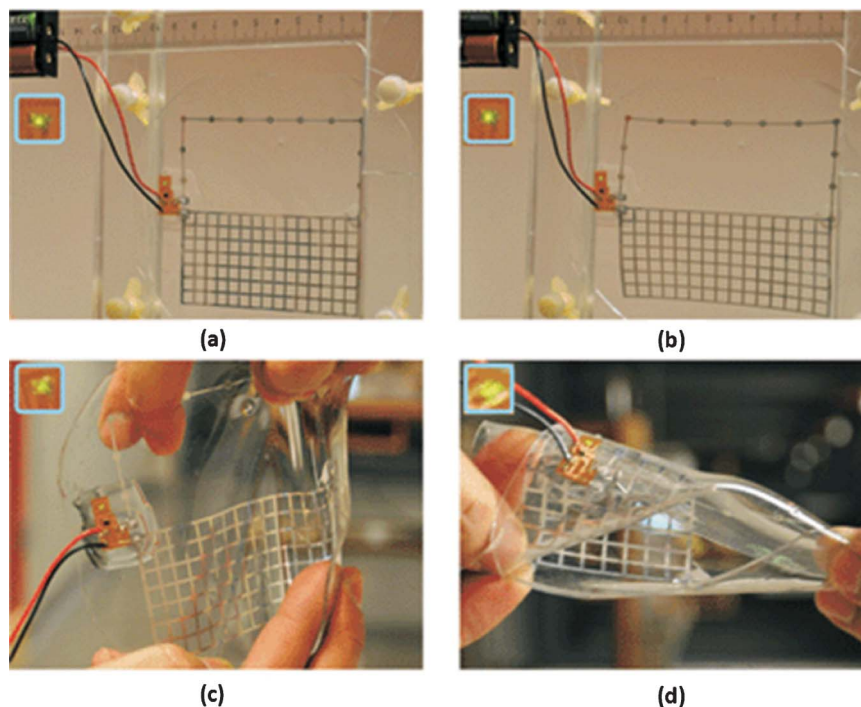
Fig. 2 Flexible microfluidic radiation sensor: (a) unstretched, (b) stretched with 15% elongation in the horizontal direction, (c) under manual applied strain in both the horizontal and vertical directions, and (d) under severe twisting. Images reproduced from ref. 8.
