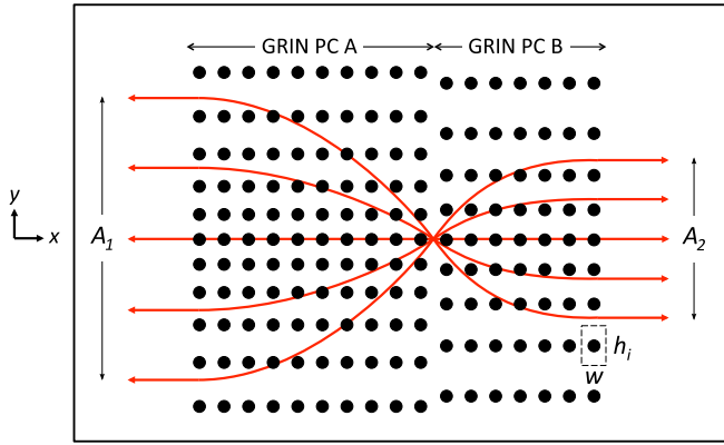
FIG. 1. Schematic of the acoustic beam aperture modifier design composed of two butt-jointed, two-dimensional GRIN PCs with different gradient profiles. The black dots represent the locations of steel cylinders, and the background material is epoxy. The aperture of a planar SV-mode BAW can be modified from wide-to-narrow or narrow-to-wide.
