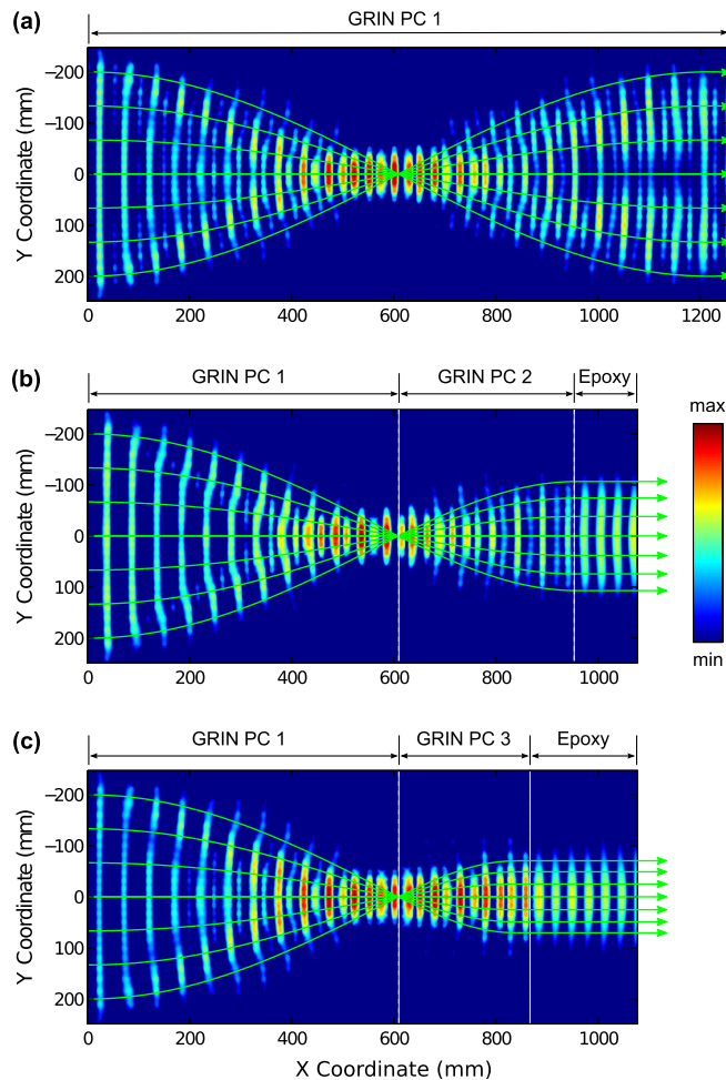
FIG. 3. FDTD-simulated acoustic wave propagation in (a) GRIN PC 1, (b) GRIN PC 1 + GRIN PC 2, and (c) GRIN PC 1 + GRIN PC 3 at the design frequency of 17.78 kHz ( \Omega = 0.25 ). The line-source-width is 400 mm wide and the wave aperture at the output is (a) maintained, (b) 210 mm, and (c) 140 mm.
