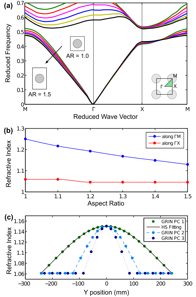
FIG. 2. (a) Band structures of rectangular-lattice steel/epoxy PC with different aspect ratios for the SV-mode BAW. (b) Refractive index of the steel/epoxy PC along \Gamma X and \Gamma M orientations against aspect ratio at reduced frequency of 0.25. (c) Effective refractive index profiles of three different GRIN PCs. Each can be fitted perfectly with a hyperbolic-secant function.
