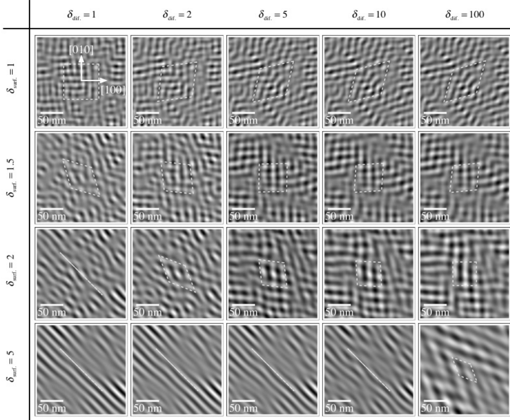
Figure 2: “Simulated” film heights for various values of \delta_{\text{dif.}} and \delta_{\text{surf.}} corresponding to \sigma(\mathbf{k}) 's appearing in Fig. 1. All figures oriented with [100] horizontal ( \rightarrow ) and [010] vertical ( \uparrow ). Dashed lines show mean grating or roll alignment predicted by \sigma(\mathbf{k}) .
