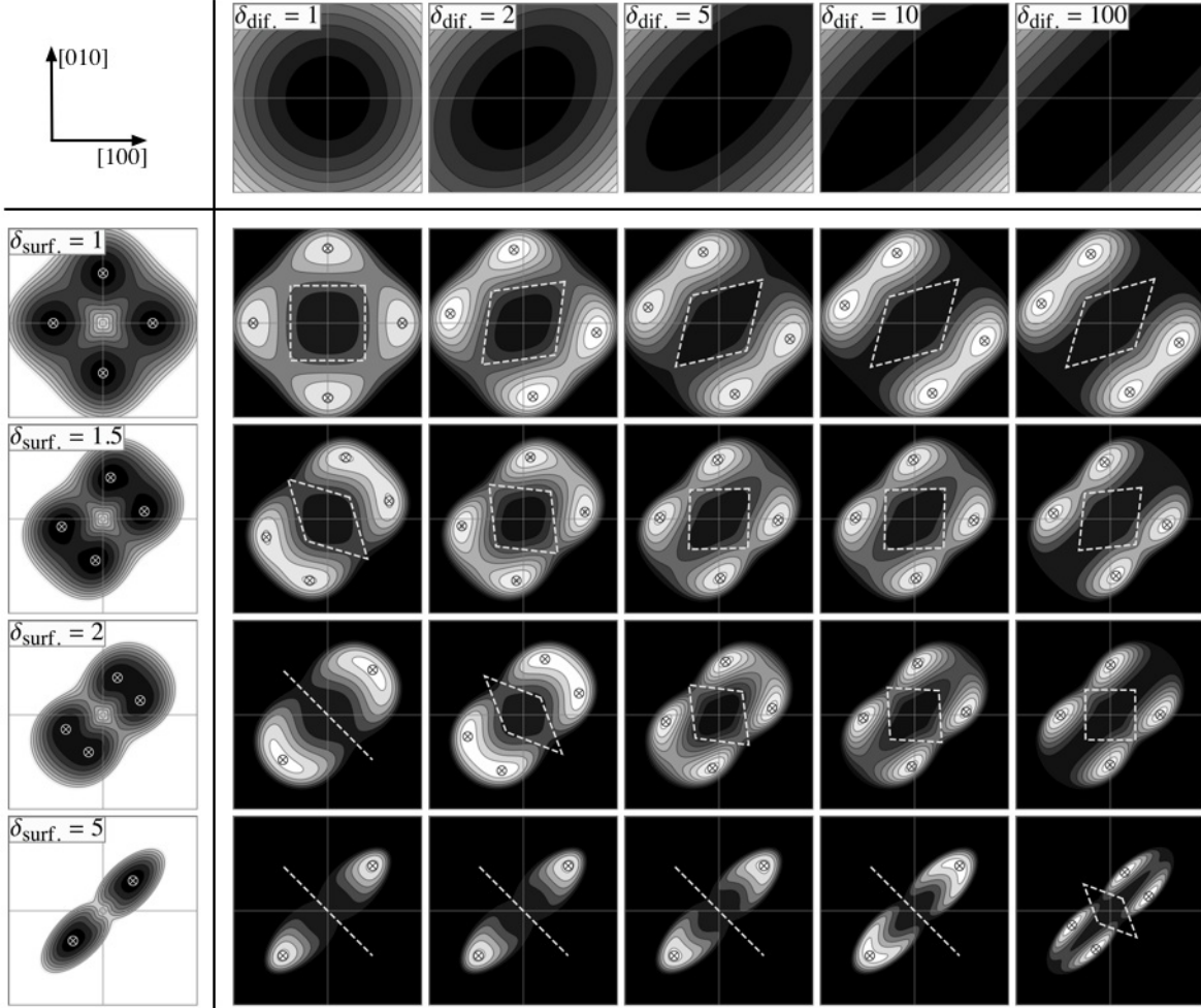
Figure 1: Graphical “multiplication table” showing effects of diffusional and surface energy anisotropy. Top row shows (\mathbf{k} \cdot \mathbf{D} \cdot \mathbf{k}) / D_0 for various surface-diffusion anisotropies \delta_{\text{dif.}} . Left column shows f(\mathbf{k}) for various surface-stiffness anisotropies \delta_{\text{surf.}} . Interior grid shows resulting dispersion relation \sigma(\mathbf{k}) (Eq. 1). Horizontal direction ( \rightarrow ) is [100] . Vertical direction ( \uparrow ) is [010] . All axes span \pm 1 rad/nm. \otimes 's indicate \mathbf{k}_E for f(\mathbf{k}) and \mathbf{k}_0 for \sigma(\mathbf{k}) plots. Dashed lines perpendicular to \mathbf{k}_0 indicate mean alignment of grating rows or rolls (Fig. 2).
