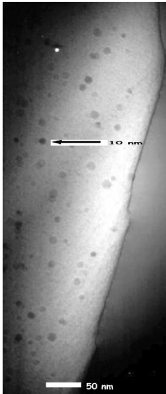
Fig. 2. TEM micrograph of photolyzed sample after cor dating the glass at 1200 °C.
