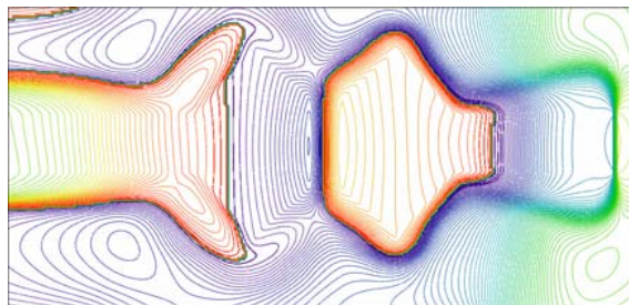
Phase Diagram with negative phase velocity
