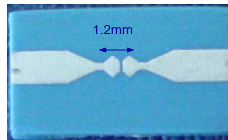
Backward-wave Transmission Line
